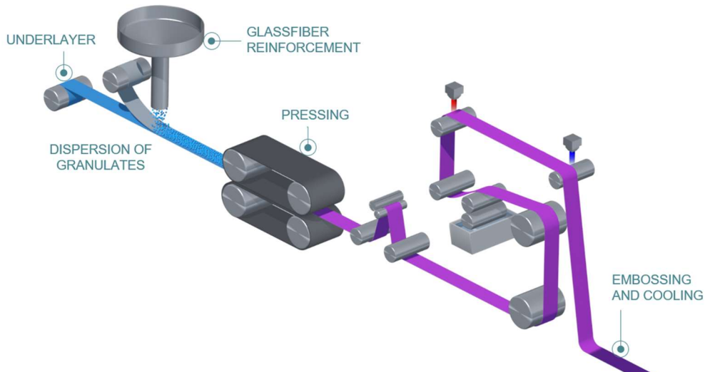
Figure 1: Pressing production process diagram
